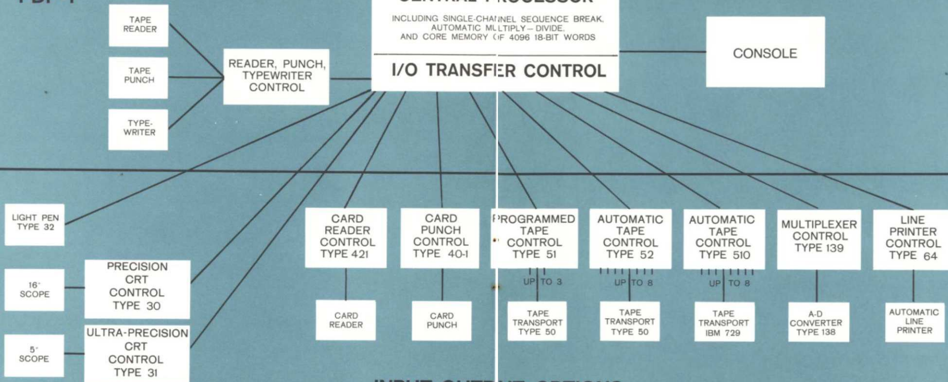
PDP-1 System Block Diagram
